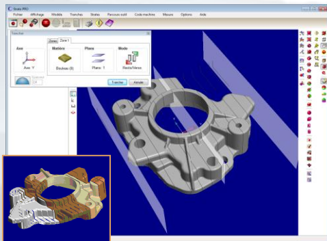
Figure 11 : Plans de tranchage
